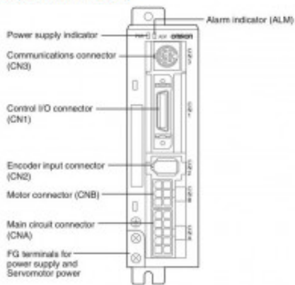
Servo Drive (100 - 400 W models)
